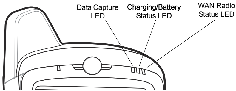
Figure 2-3 LED Indicators
