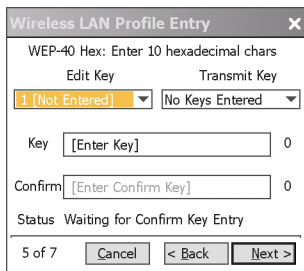
Figure 5-6 WEP-40 WEP Keys Dialog Box
