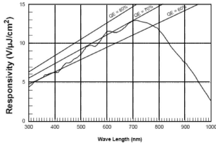
M5xx Spectral Response (excludes lens and light source characteristics)
